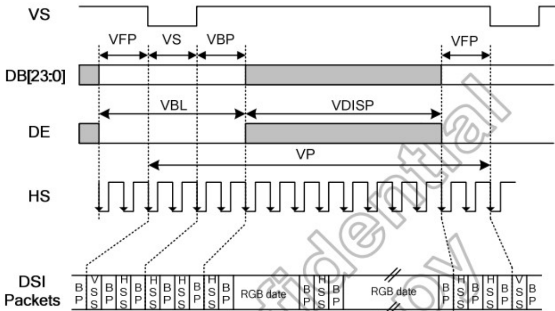
Figure 8.10: Vertical timings for DSI I/F
