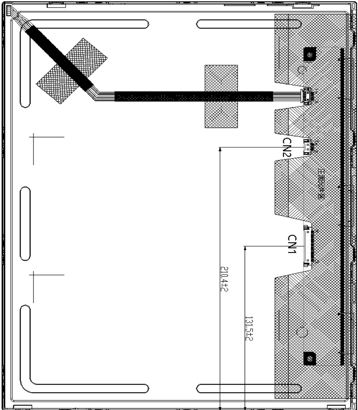
< Figure 4.TFT-LCD Module Outline Dimensions (Rear View) >
