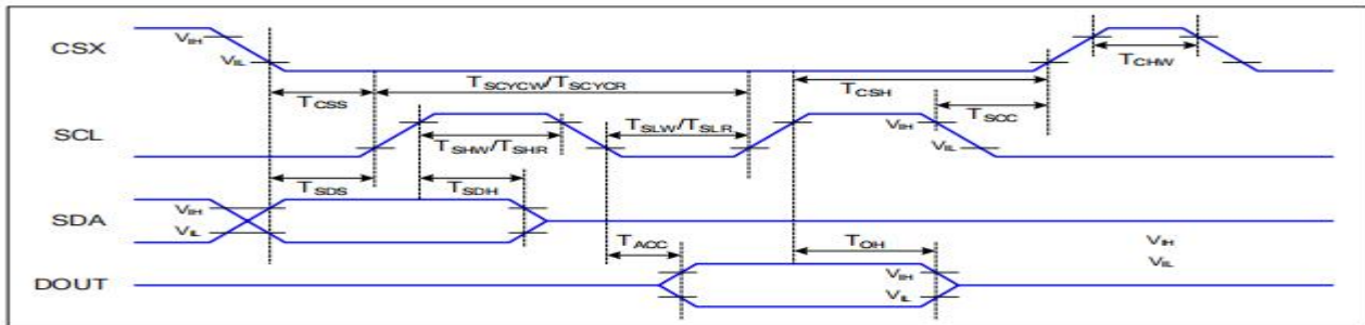
Figure 1 3-line serial Interface Timing Characteristics
