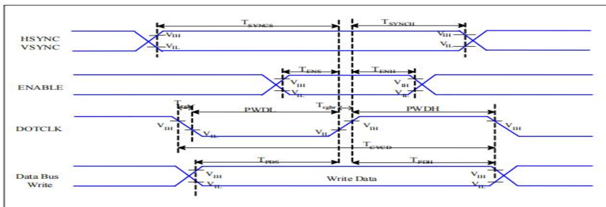
Figure 3 RGB Interface Timing Characteristics
