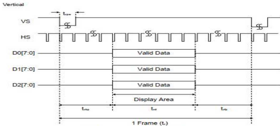
Figure 43 Vertical Input timing at sync mode.
