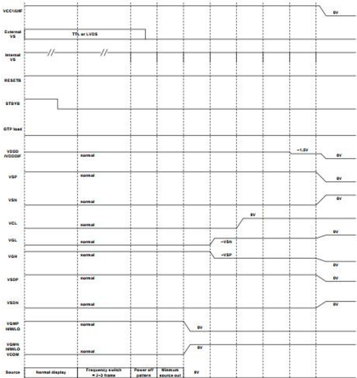
Figure 25 Power off sequence external mode.
