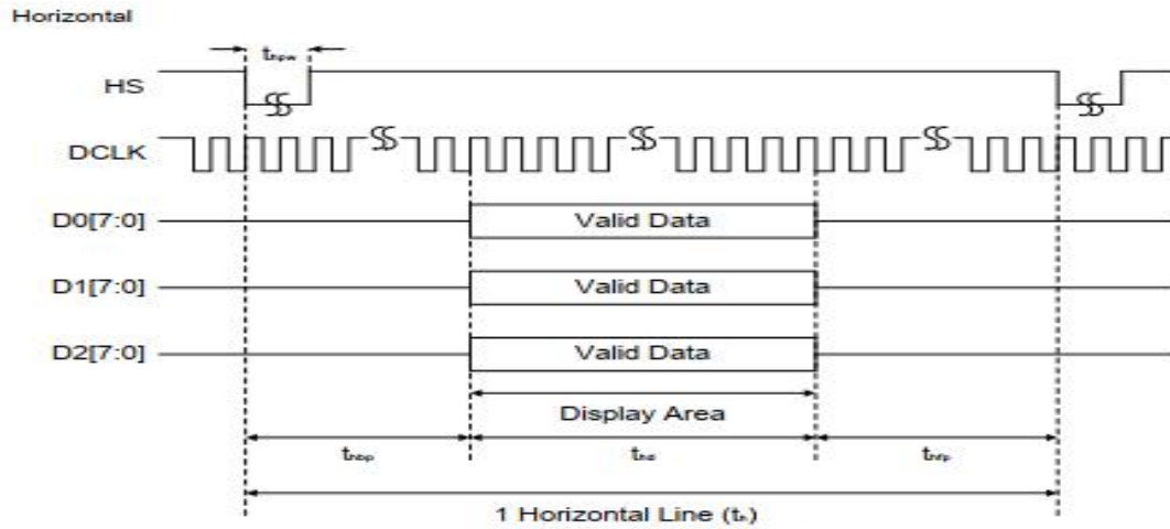
Figure 42 Horizontal Input timing at sync mode.
