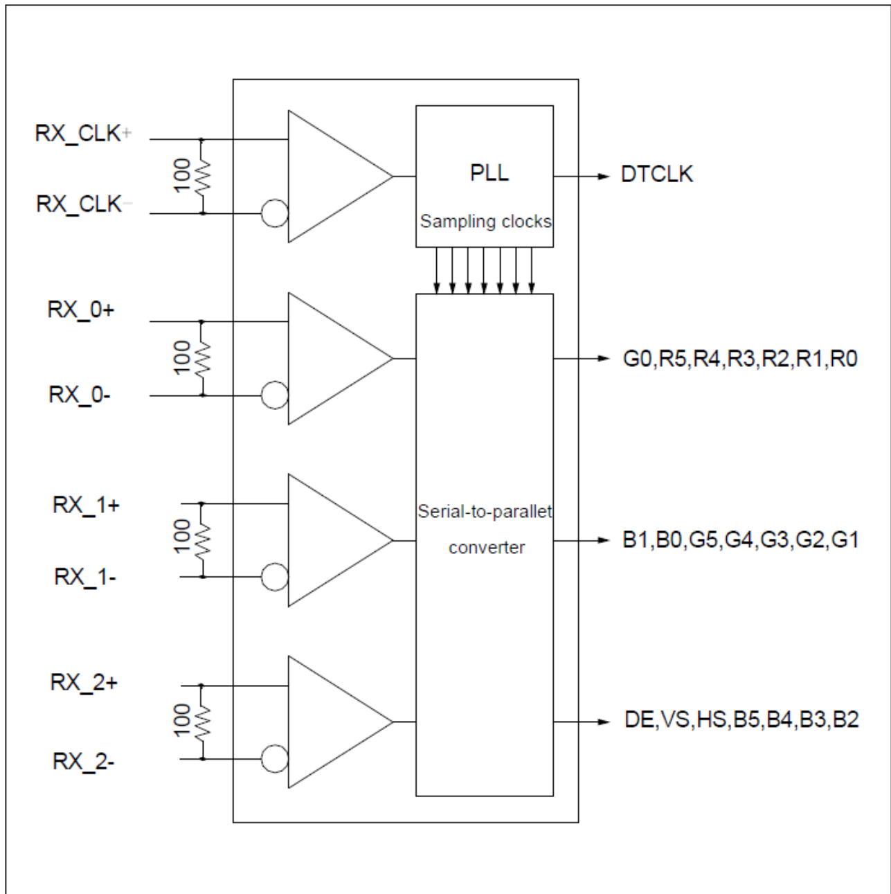
Figure 10 LVDS Receiver Internal Circuit
